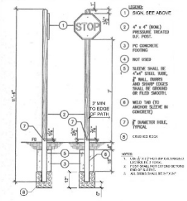
5 SLO COUNTY SIGN POST STANDARD NTS 349161-05
