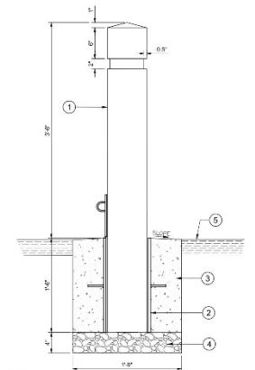
1 ASPHALT PATH 1/32" = 1'-0" 33219-01 2 LODGE POLE FENCE NTS 33219-01-02
