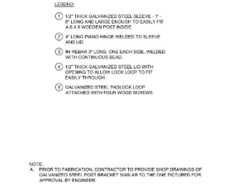
4 REMOVEABLE WOOD BOLLARD BRACKET NTS 129338-10
